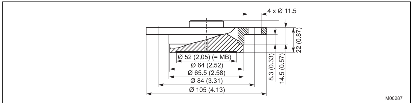
Fig. 9: Dimensions in mm (inches)
