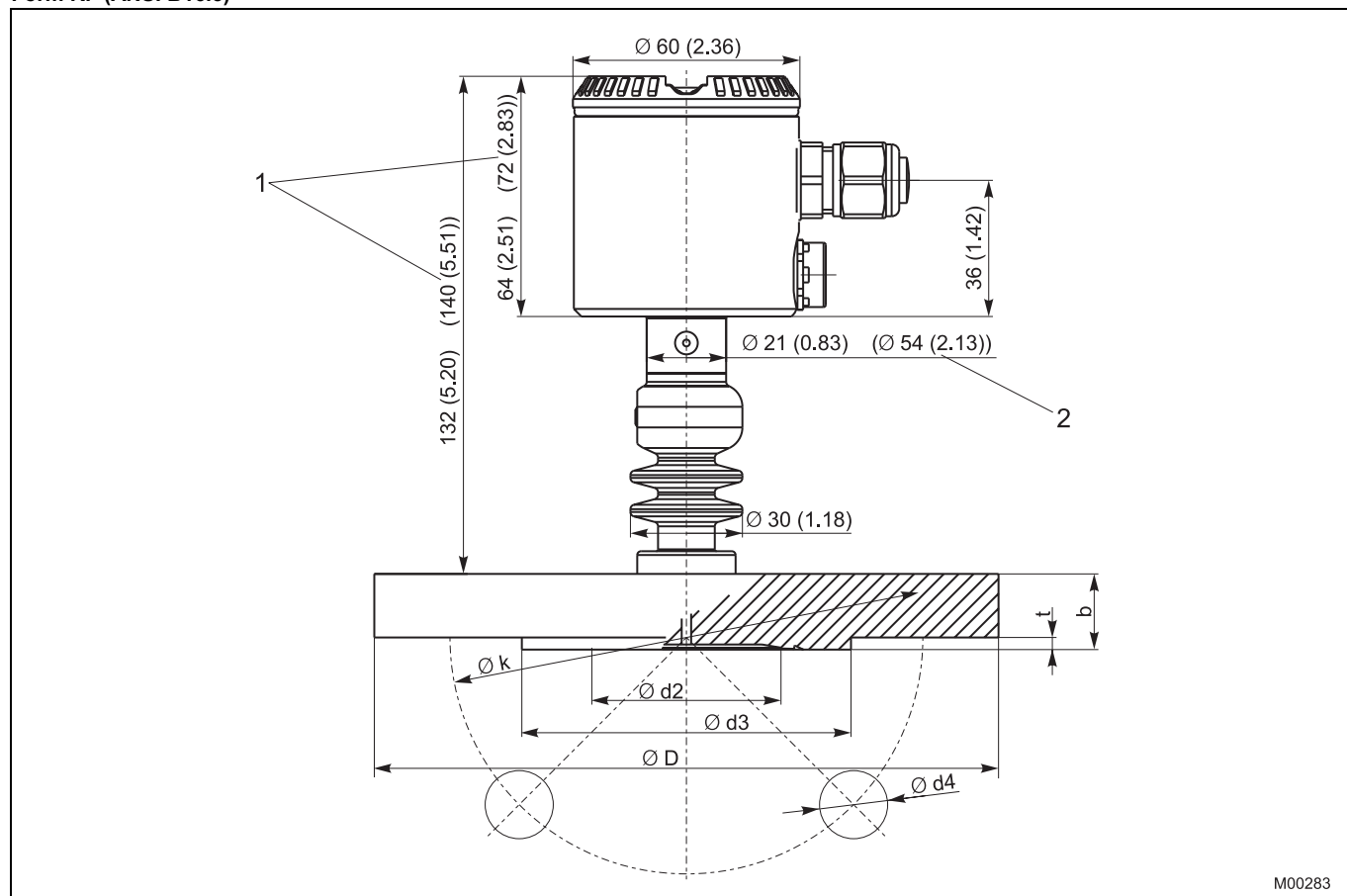
Fig. 3: Dimensions in mm (inches)
