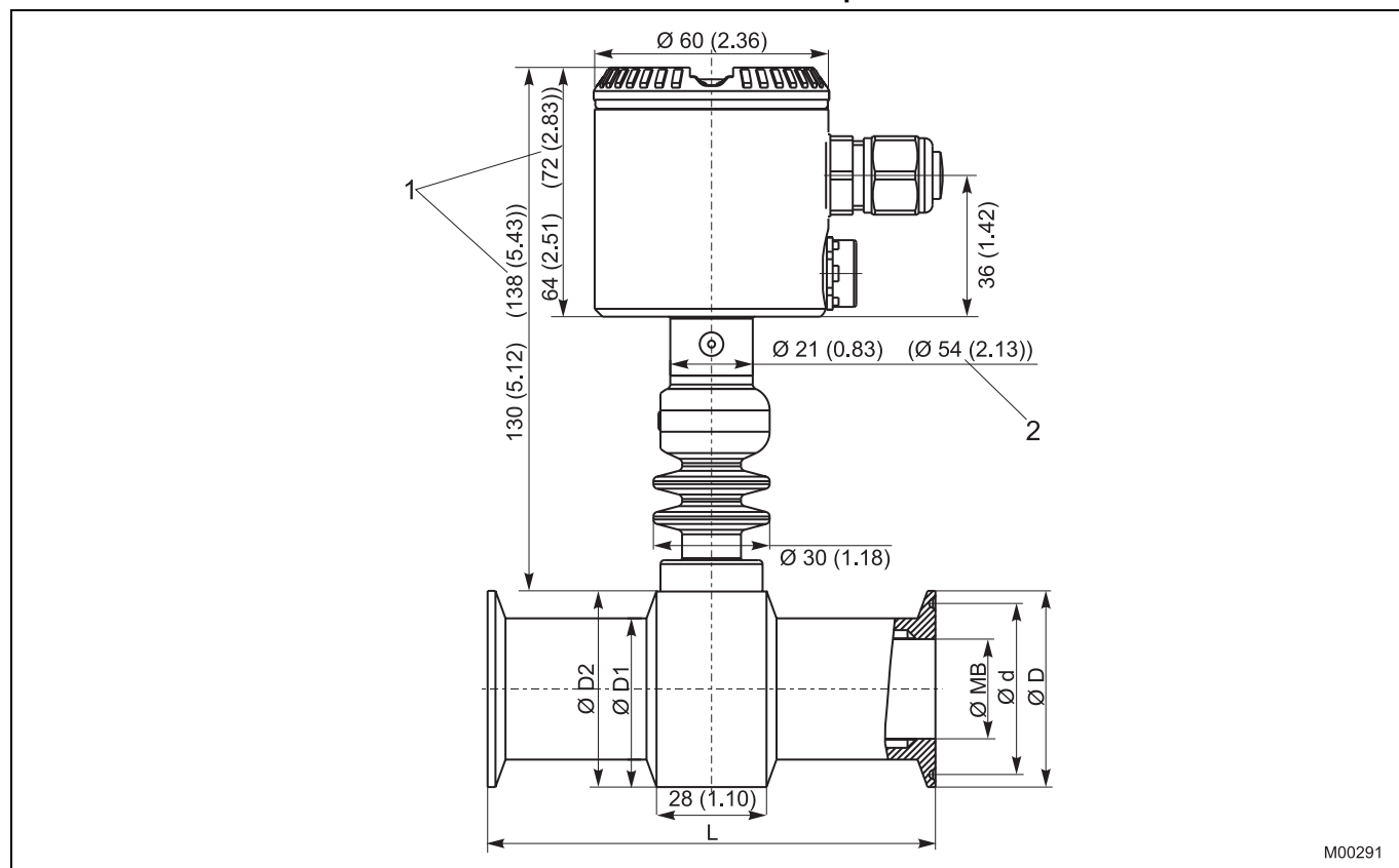
Fig. 13: Dimensions in mm (inches)
