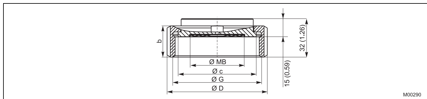
Fig. 12: Dimensions in mm (inches)
