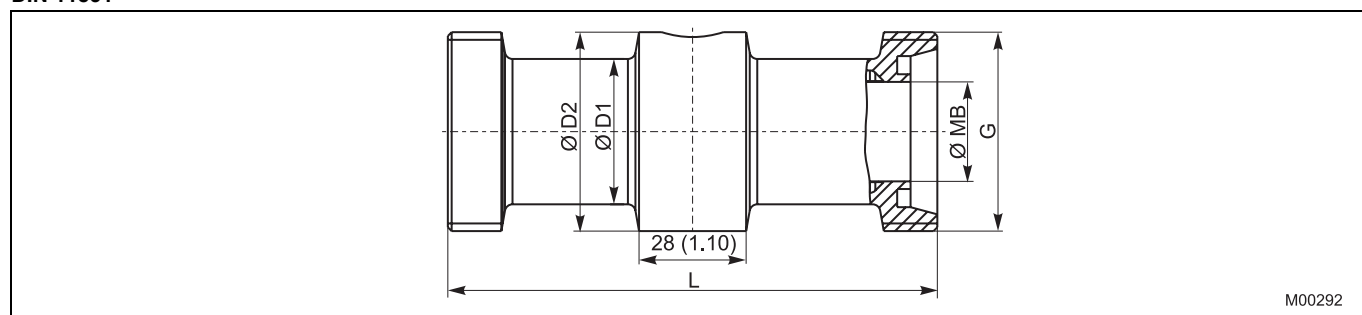
Fig. 14: Dimensions in mm (inches)
