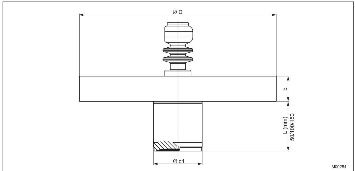
Fig. 4: Dimensions in mm (inches)
