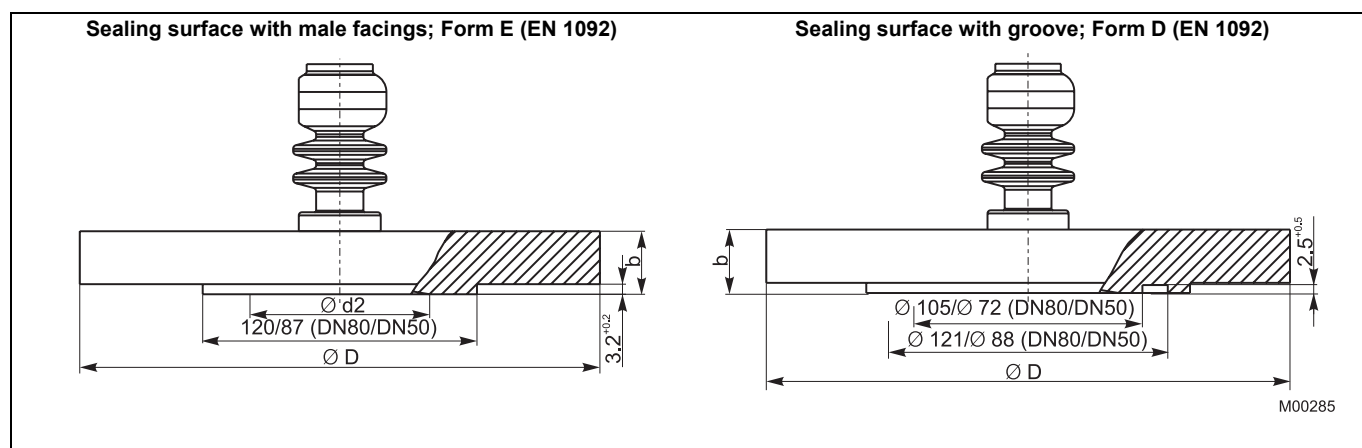
Fig. 5: Dimensions in mm (inches)
