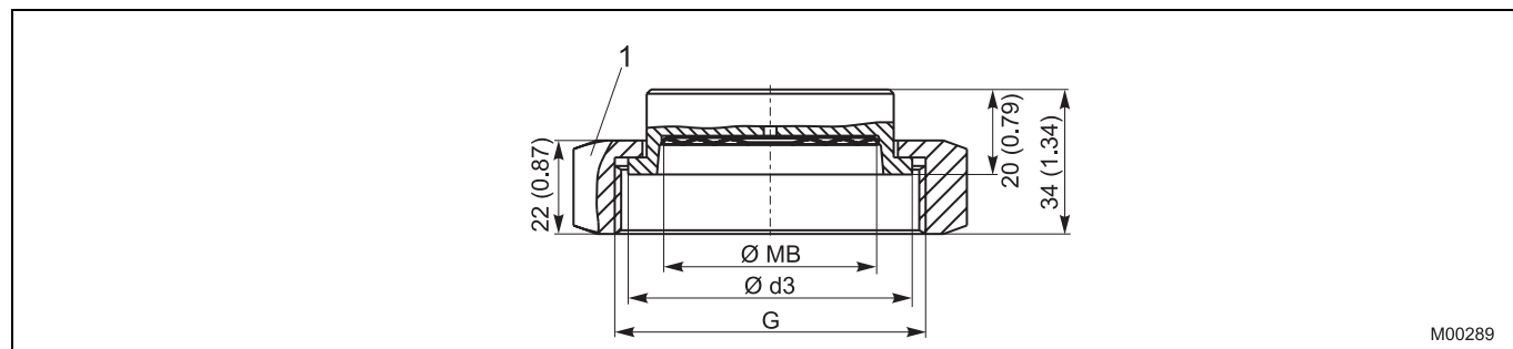
Fig. 11: Dimensions in mm (inches)
