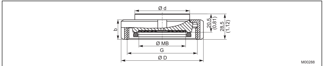
Fig. 10: Dimensions in mm (inches)
