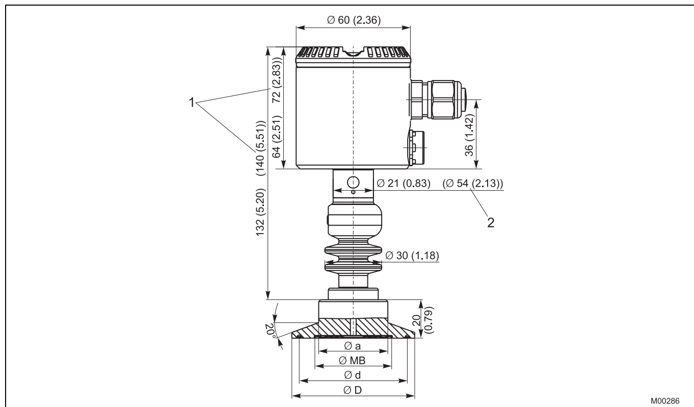
Fig. 6: Dimensions in mm (inches)
