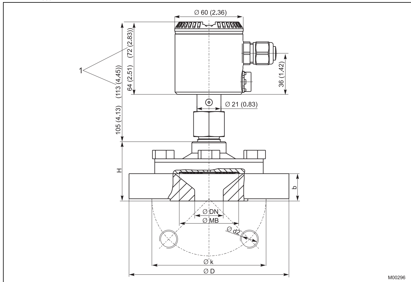
Fig. 17: Dimensions in mm (inches)
