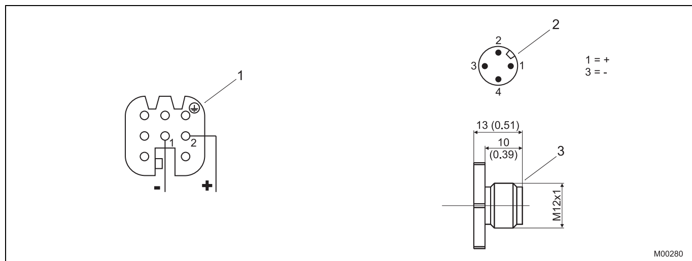
Fig. 20: Dimensions in mm (inches)
