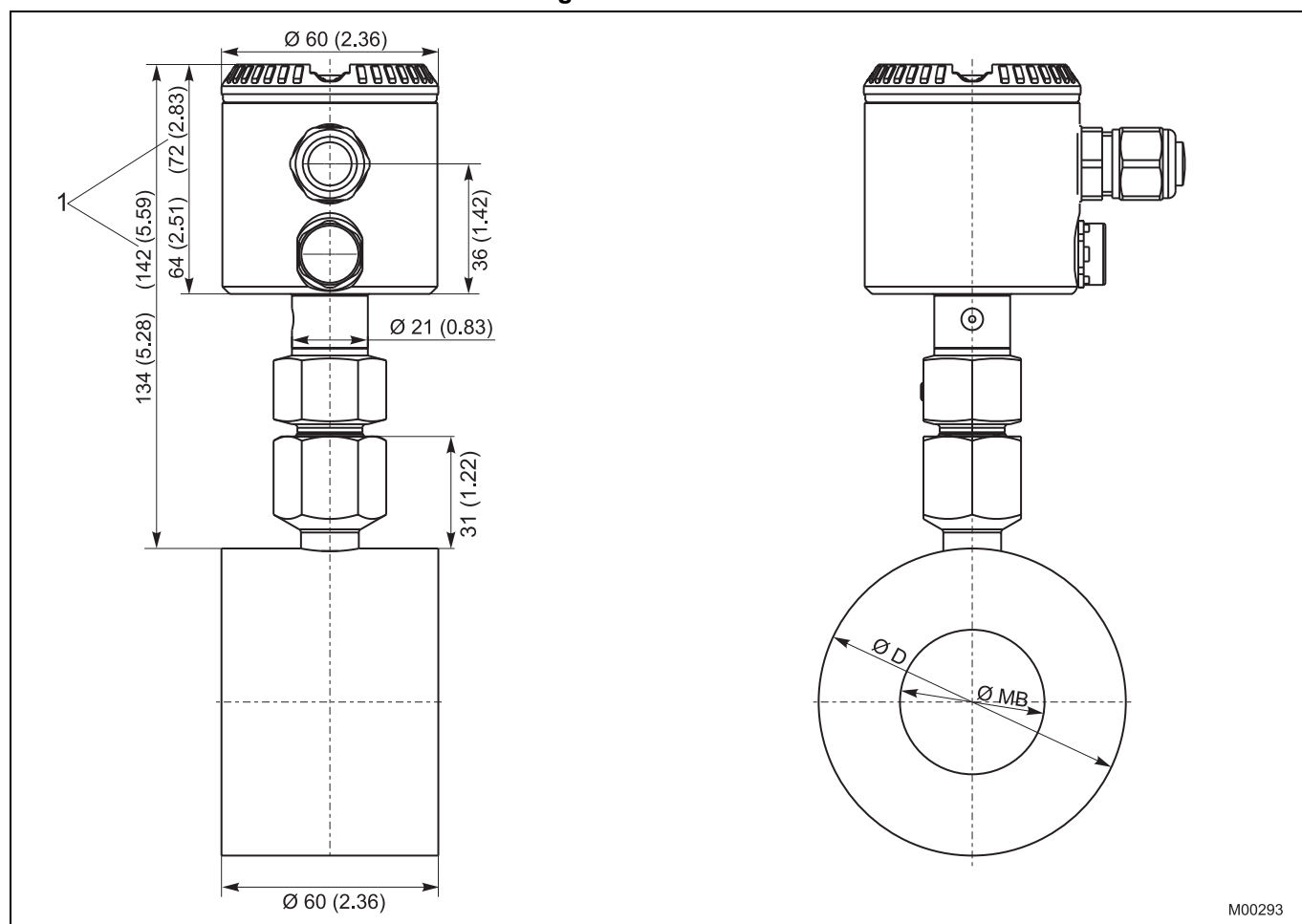
Fig. 15: Dimensions in mm (inches)
