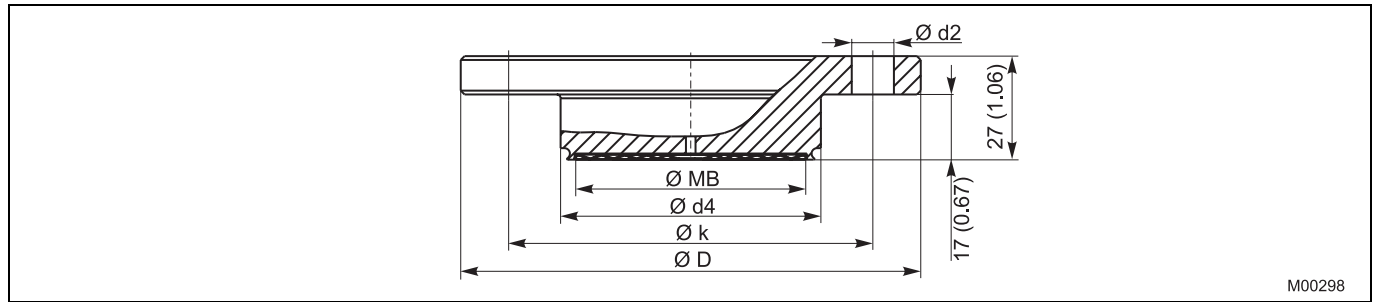
Fig. 8: Dimensions in mm (inches)
