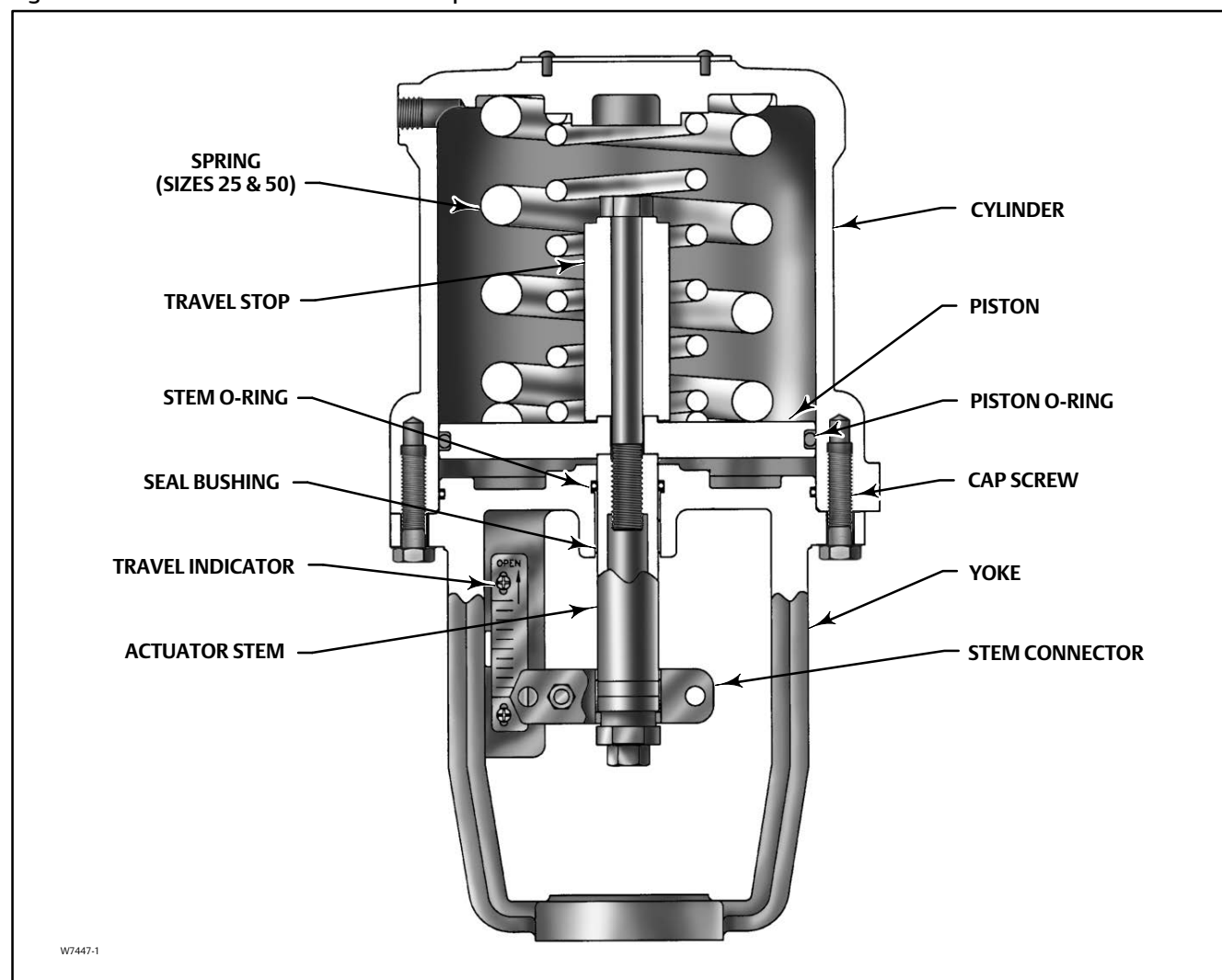
Figure 1. Fisher 585C Piston Actuator Components
