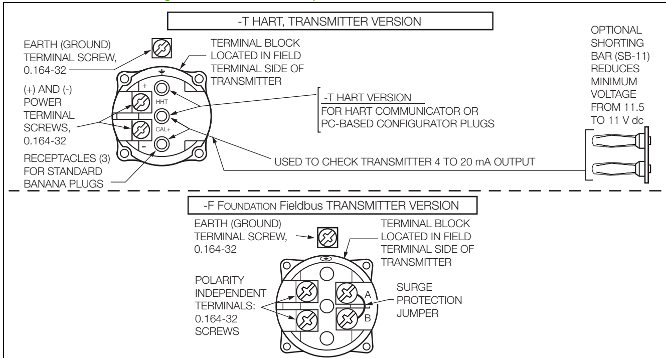
Figure 22. Field Terminals Compartment for HART and Fieldbus
